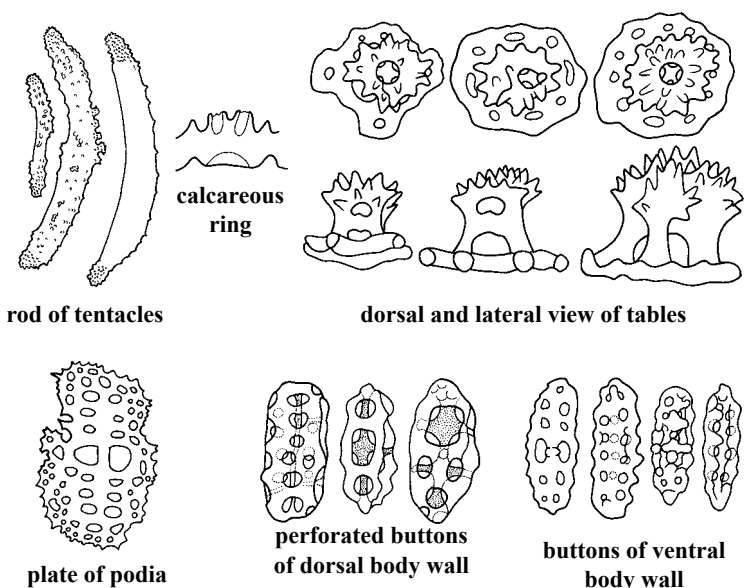
(after Cherbonnier, 1988)
