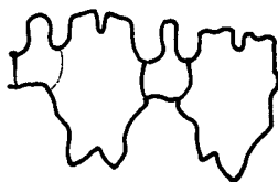
calcareous ring
