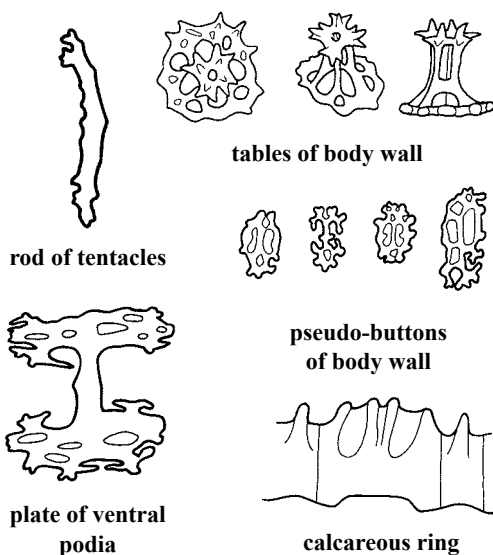
(after Cherbonnier, 1980)
