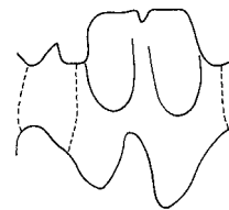
calcareous ring
