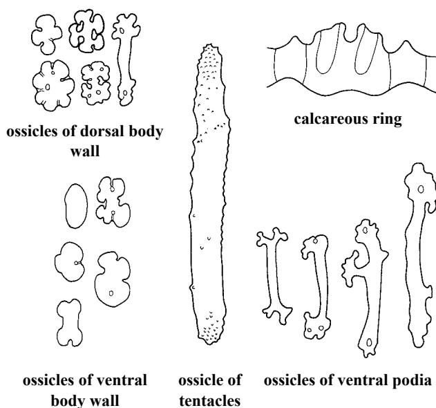
(after Cherbonnier, 1988)
