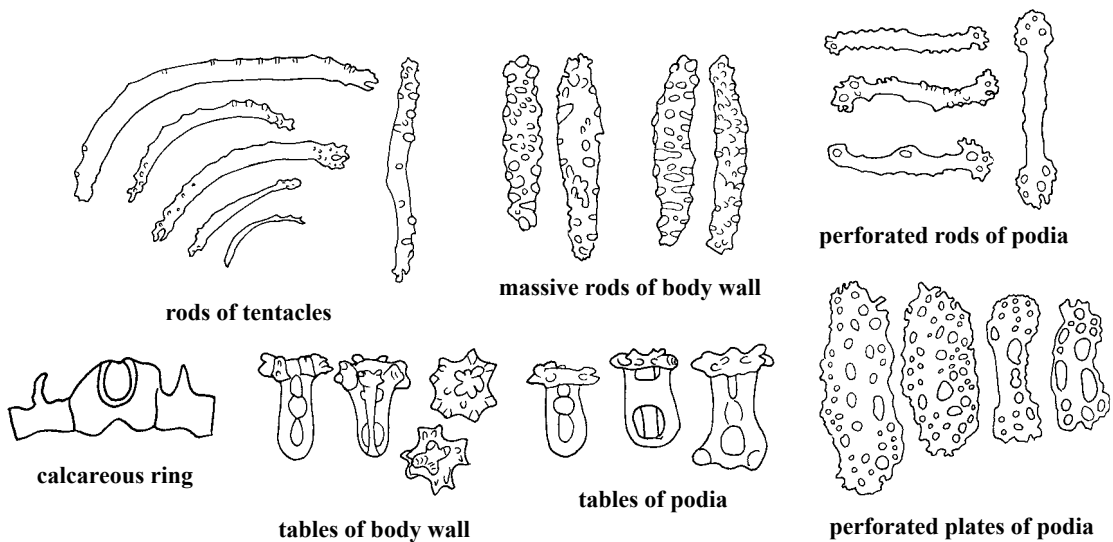
(after Massin, 1999)
