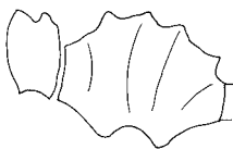
calcareous ring
