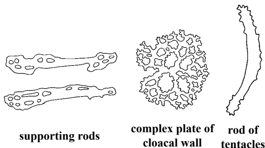
(after Liao, 1980)
