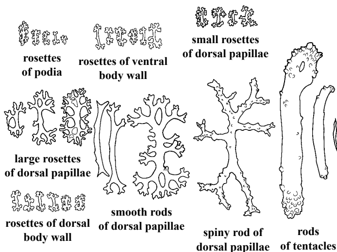
(after Massin, 1996)
