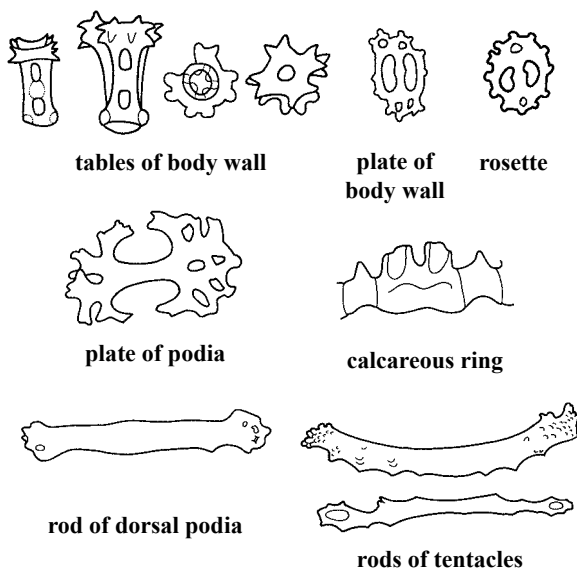
(after Cherbonnier, 1980)
