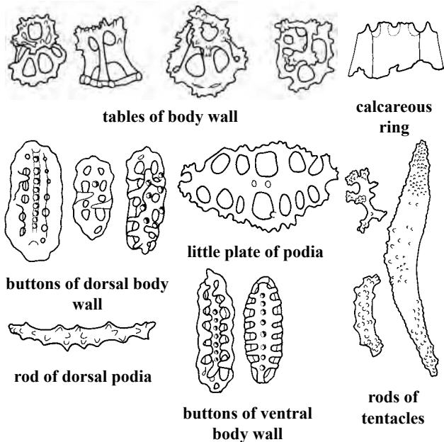
(after Cherbonnier, 1980)
