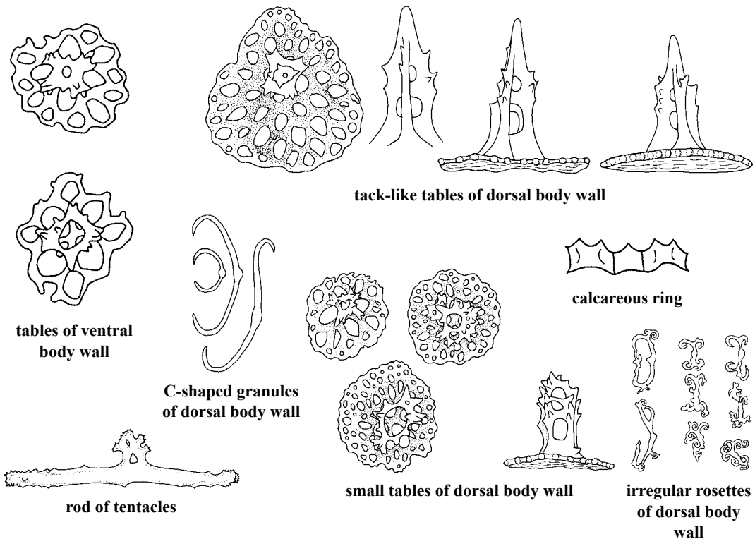
(after Cherbonnier, 1967)
