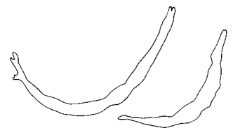
curved rods
