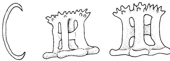
C-shaped rod
